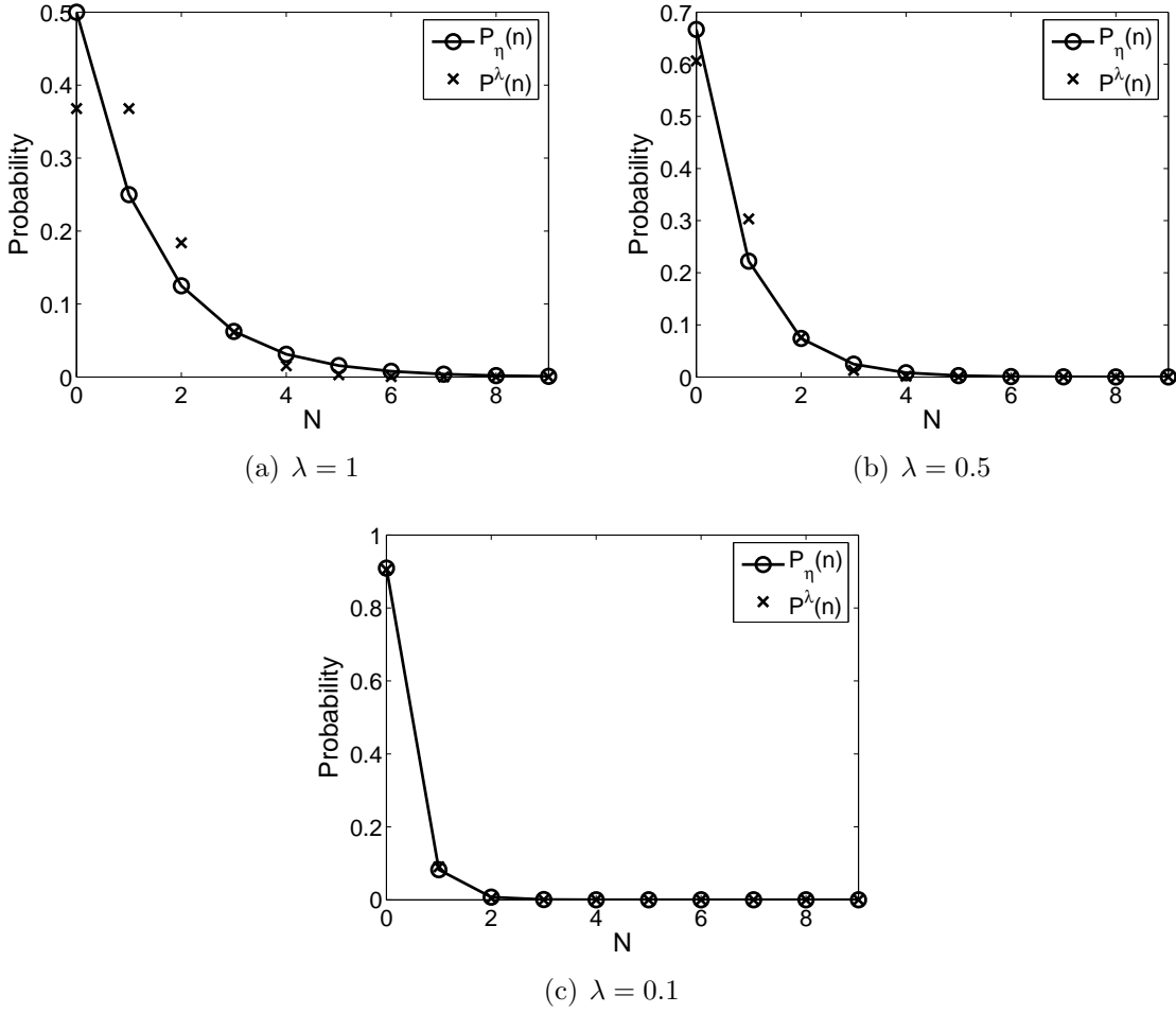
Figure 1. Comparison between P_\eta(n) and P^\lambda(n) . P_\eta(n) is computed by Eq. (1) with a given P(N) , which is a Bose-Einstein distribution with expectation being 100. We choose \eta to be \lambda/100 for (a) \lambda = 1 ; (b) \lambda = 0.5 and (c) \lambda = 0.1 , respectively. P^\lambda(n) is the corresponding Poisson distribution with parameter \lambda . P_\eta(n) (represent as 'o's) and P^\lambda(n) (represent as 'x's) are plotted for n = 0, 1, \dots, 9 (since P_\eta(n) and P^\lambda(n) are neglecting small for big n ). We can see for \lambda = 1 and 0.5 the difference between P_\eta(n) and P^\lambda(n) is evident. However, for \lambda = 0.1 , the Poisson distribution P^\lambda(n) makes a very good approximation to P_\eta(n) .
